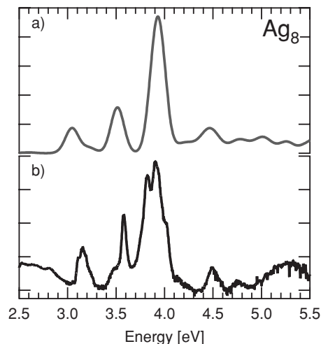
FIG. 3. Comparison between the experimental spectra and the calculated ones for \text{Ag}_8 : (a) superposition of both calculated isomers with adjusted weight; (b) experimental spectrum obtained in argon.
