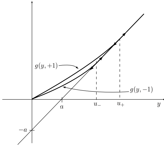
Figure 4: The functions g(\cdot, \pm 1) under the hypotheses of Theorem 16. The arrows indicate the presence of smooth fit.
