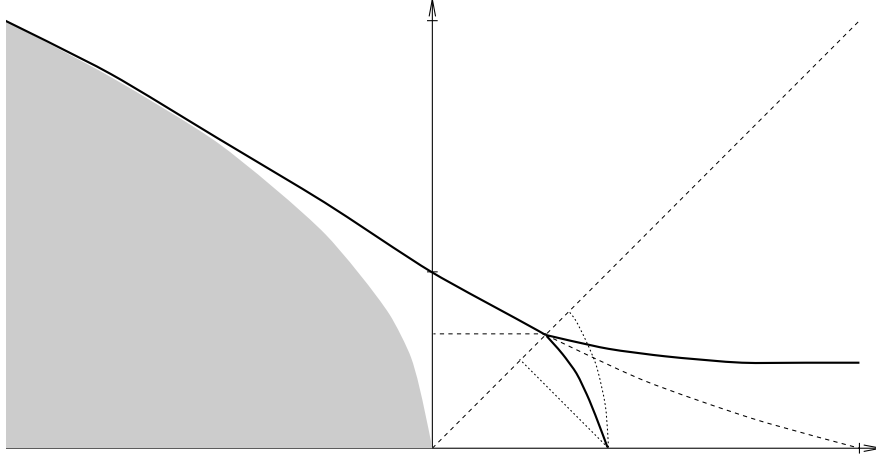
Figure 2: Schematic representation of the phase diagram in the plane \tanh J_{\sigma\tau} versus \tanh J_{\sigma} = \tanh J_{\tau} . We have indicated the critical lines (solid lines), and the self-dual line (which coincides with the solid line up to the splitting and then follows the dashed line). The shaded region corresponds to the set of parameters at which the random-cluster representation is not available. The estimates of the location of the critical line are also shown (dotted lines).
