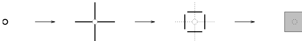
Figure 1: Lattice transformations (only one site shown)
