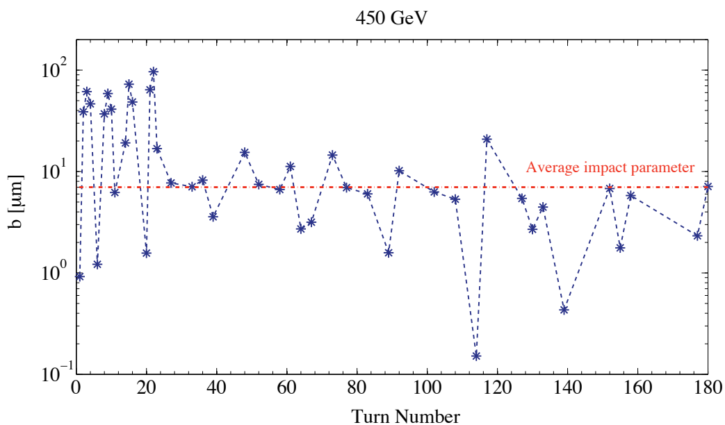
Figure 5.7: Impact parameter b as a function of the number of turns for the b = 1\ \mu\text{m} at first turn case, injection energy and Beam 1 horizontal halo. Only the particles interacting for the first time with the collimator are considered.
