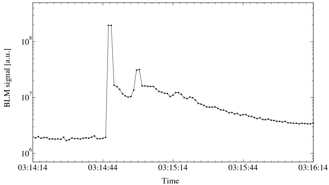
Figure 7.16: Zoom of the BLM signal versus time after a change in the horizontal tune at 3:14:45. An unexplained second loss peak appeared, also seen during other measurements.
