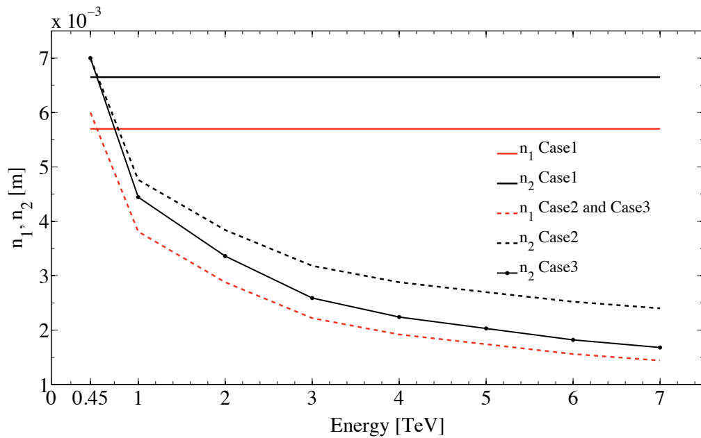
Figure 6.18: The half gaps of the IR7 TCPs ( n_1 ) and TCSGs ( n_2 ) are shown as a function of the beam energy for the proposed settings. Case 1 refers to the constant and case 2 to the tolerance optimized settings. In case 3 the collimator gaps are scaled with \sqrt{\gamma} .
