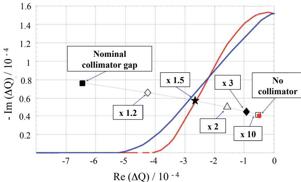
Figure 6.12: Stability limits at top energy as a function of the collimator openings: nominal collimator gap (black squares), no collimators (red circle), and intermediate situations where the collimator gap is increased by 20%, 50%, a factor of 2, 3 and 10 [60].
