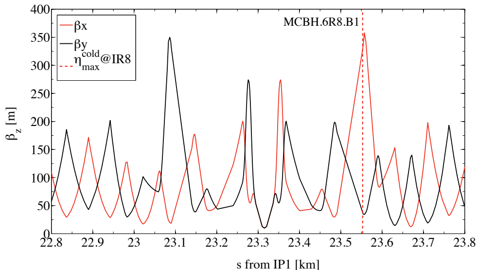
Figure 6.2: \beta_x and \beta_y functions around IP8. The location of \tilde{\eta}_{max}^{cold} the Beam 1 horizontal halo at injection energy is shown. The optics around IP8 is asymmetric and the \beta -function reaches its maximum downstream of the interaction point.
