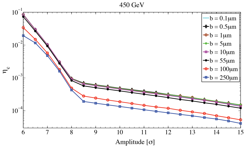
Figure 5.8: Inefficiency curves for impact parameters at first turn varying from 0.1 \mu\text{m} up to 250 \mu\text{m} . The statistical error is within the marker width.
