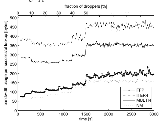
Fig. 2. Bandwidth usage per message delivery. Setup as in Fig. 1. Iterative and multipath routing relies on 4-way message redundancy for fault-tolerance, which results in high bandwidth usage. FFP's only overhead are the feedback messages, which are small in size and can be sent in bulk.
