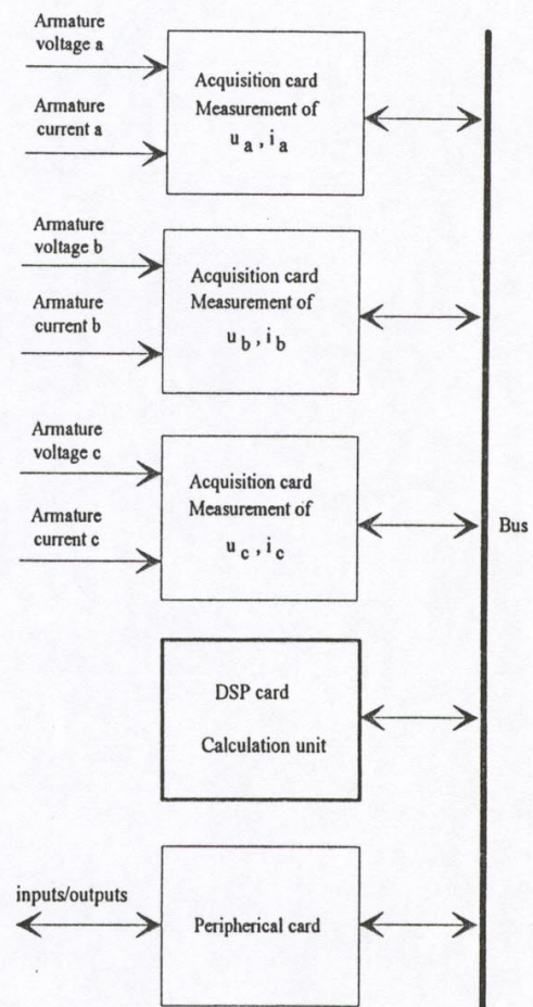
Fig. 1 : Synoptic diagram
