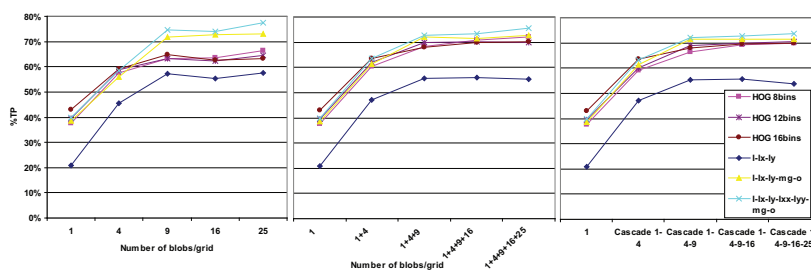
Fig. 7. %TP on the 1st Data set (pedestrians only) for various region descriptors based on 3 Object descriptors: Left hand-side: A single grid of n blobs (here n=1,4,9,16,25 ). Middle column: collection of grids. Right hand-side: Cascade of grids.
