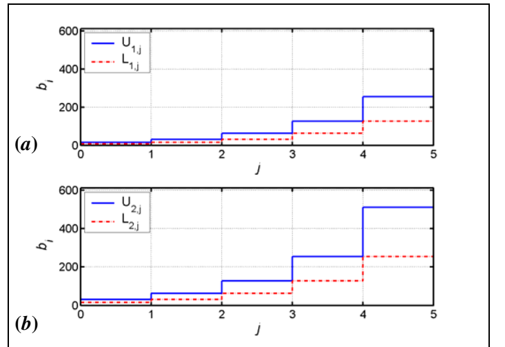
Figure 4. Back-off selection ( b_i ) as a function of the back-off stage ( j ) for CLD_3 and nodes in: (a) C_1 , (b) C_2 .
