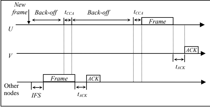
Figure 2. 802.15.4 Medium Access Data Transmission.
