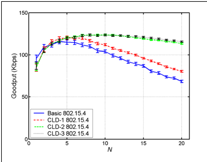
Figure 5. Goodput.
