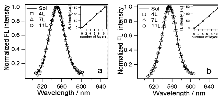
Figure 2. Steady-state fluorescence spectra of CdSe (a) and CdSe@CdS (b) QDs in films at n = 4, 7 , and 11 . The solid lines represent the emission in solution. The insets show the emission intensity vs the number of bilayers.
