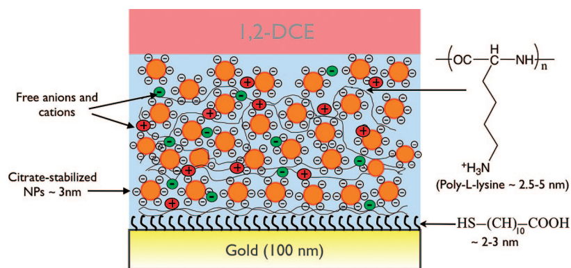
Scheme 1. Schematic representation of the ultrathin film (pLys/NPs) n assembled on MUA-modified-gold substrate.
