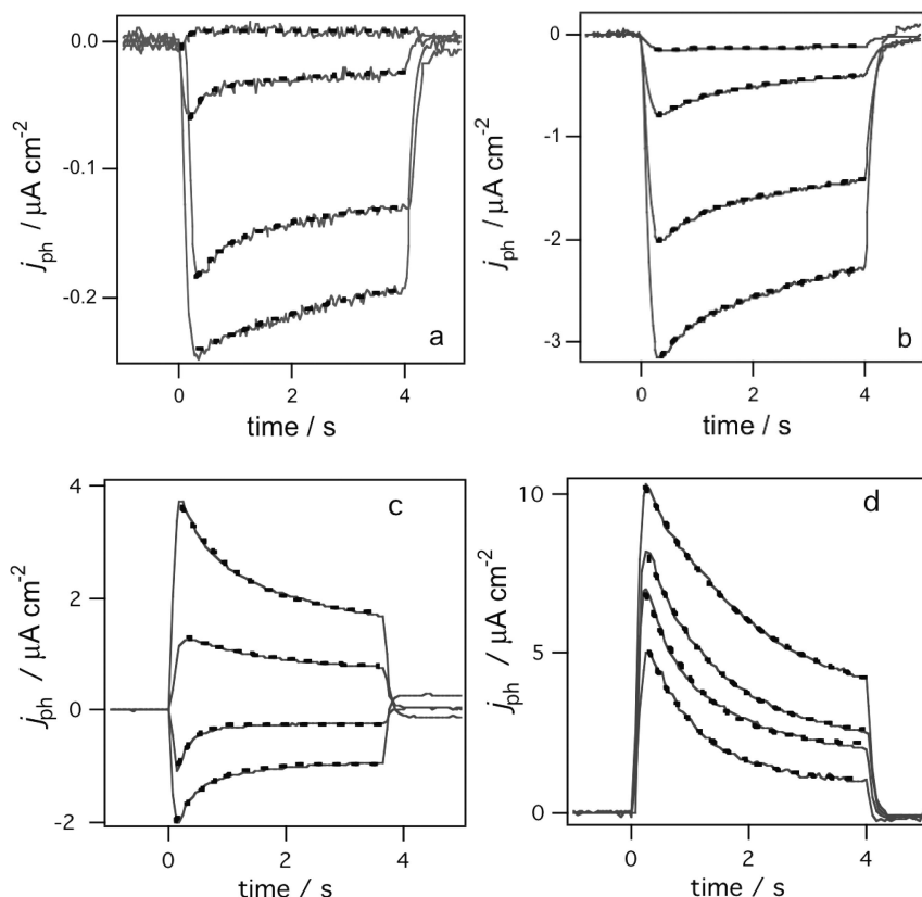
Figure 5. Photocurrent transient responses of (pLys/CdSe) 1 (a), (pLys/CdSe) 7 (b), (pLys/CdSe@CdS) 1 (c), and (pLys/CdSe@CdS) 7 (d) at four different potentials: -0.4, 0, 0.4, and 0.8 V from bottom to top. The dashed lines are fittings employing eq 7.
