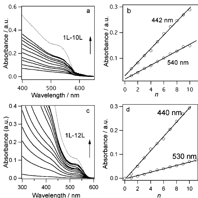
Figure 1. UV–vis absorption spectra of alternating film deposition of (pLys/CdSe) n bilayers (a) and (pLys/CdSe@CdS) n bilayers (c). The dotted lines in panels a and c represent the absorption spectra of CdSe and CdSe@CdS dispersions in aqueous solutions, respectively. Shown are the absorbances at the indicated wavelengths vs the number of bilayers n of CdSe (b) and CdSe@CdS (d). The solid lines correspond to the linear fittings.
