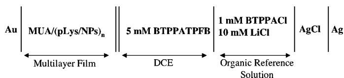
Scheme 3. Schematic illustration of the electrochemical cell and electrolyte compositions.
