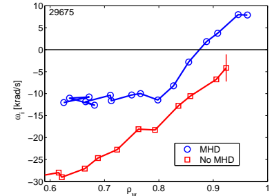
Figure 4: Comparison of edge rotation profiles with and without MHD mode
