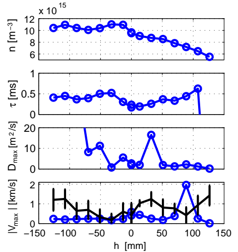
Figure 4: Values of n , \tau , D_{max} and V_{max} Vs vertical position. The convective velocity V_{max} (blue line) is compared with the plasma ExB velocity (black line).
