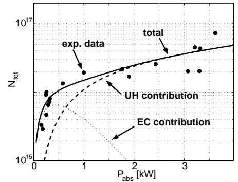
Figure 2: Dots: total number of plasma particles Vs absorbed power. Lines are a fit to determine the contributions to S(\mathbf{x}) from electrons accelerated at the EC and UH layers.
