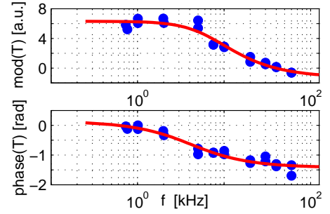
Figure 3: Dots: measured amplitude and phase of T from ion saturation current measurements Vs frequency. Solid line: fit based on a single time constant response model.
