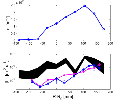
Figure 5: Top: density radial profile. Bottom: flux \Gamma from modulation experiments (dark region between maximum and minimum values estimated from D_{max} and V_{max} ), and from direct measurements of the turbulent flux integrated below (diamonds) and above (circles) 10kHz.
