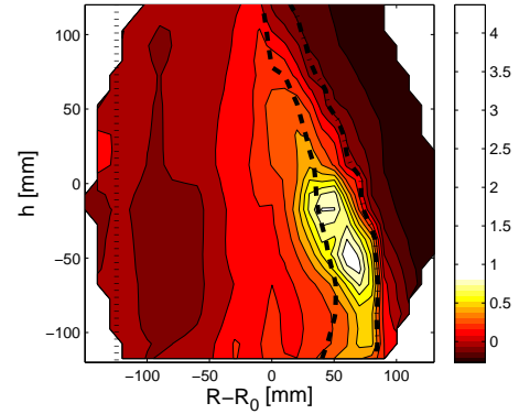
Figure 1: Relative density variation following a pulse of the injected power. Lines indicate the position of the EC (dot) and UH (dash: before pulse, dot-dash: end of the pulse) layers.
