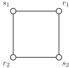
FIG. 1. An undirected graph with unit capacities on the edges. While there exist integral 2-commodity flows satisfying unit demands for terminal pairs \{s_1, r_1\} , \{s_2, r_2\} and for terminal pairs \{s_1, r_2\} , \{s_2, r_1\} , there is only a half-integral 2-commodity flow for terminal pairs \{s_1, s_2\} , \{r_1, r_2\} .
