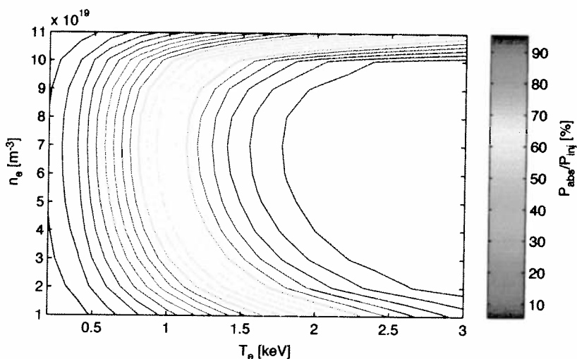
Figure 3. Assuming the 1D slab geometry and using Equation (2), the contour plot of the absorbed power fraction is shown in the density and temperature parameters domain. This shows that X3 wave can be well absorbed ( P_{abs}/P_{inj} \geq 90\% ) within the density range 3 \cdot 10^{19} \leq n_e \leq 10 \cdot 10^{19} \text{ m}^{-3} if the temperature T_e \geq 2.5 keV.
