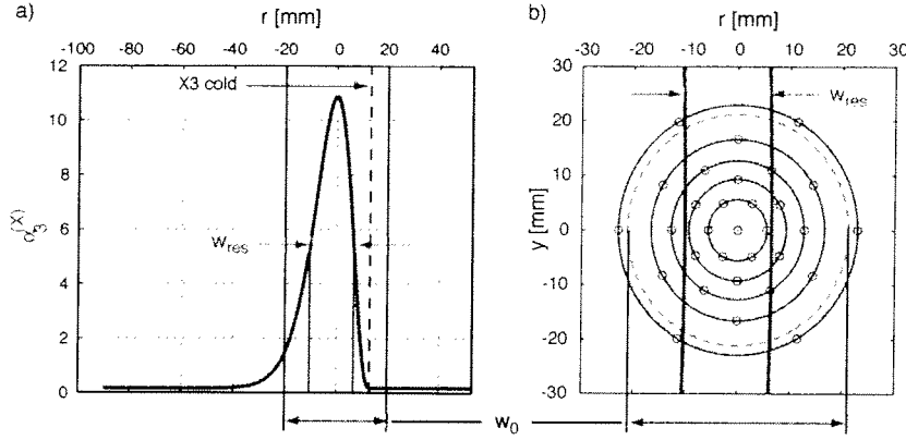
Figure 9. a) w_{res} , determined from \alpha_3^{(X)} calculated for T_e = 2 keV and n_e = 4 \cdot 10^{19} m^{-3} , is compared to the X3 beam waist w_0 . b) The ray distribution (small open circles) over the beam cross-section, where N_{rays} = 6 , N_c = 5 and N_{tot} = 31 , used in the gaussian beam model. The beam waist, w_0 (dashed line) is also shown.
