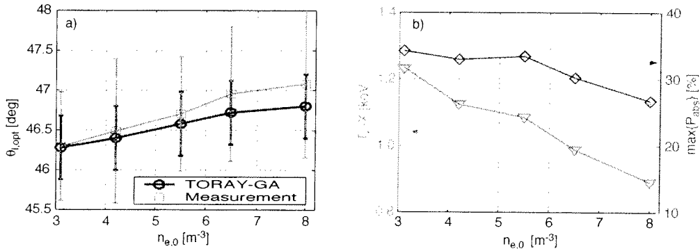
Figure 17. a) The launcher optimal angle versus the central density n_{e,0} has been obtained from T_e -X measurement (squares) and from TORAY-GA calculation (circles). The vertical bars represent \delta\theta which does not depend on the density. b) The absorbed power, calculated by TORAY-GA at \theta_{l,opt} (diamonds curve) is compared to the T_e -X signal measured at \theta_{l,opt} (triangles).
