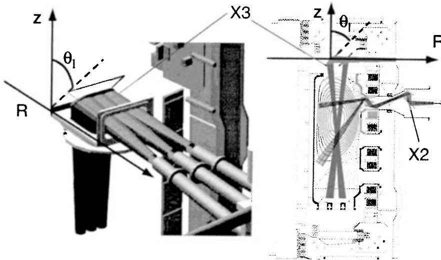
Figure 13. The poloidal view of TCV shows the launcher flexibility for vertical injection (X3) and lateral injection (X2). The X3 launcher can move in the radial direction between 800 mm and 960 mm ( R_0 = 880 mm on TCV) from shot to shot. The launcher poloidal angle \theta_l can vary in the range 40^\circ - 50^\circ during the shot.
