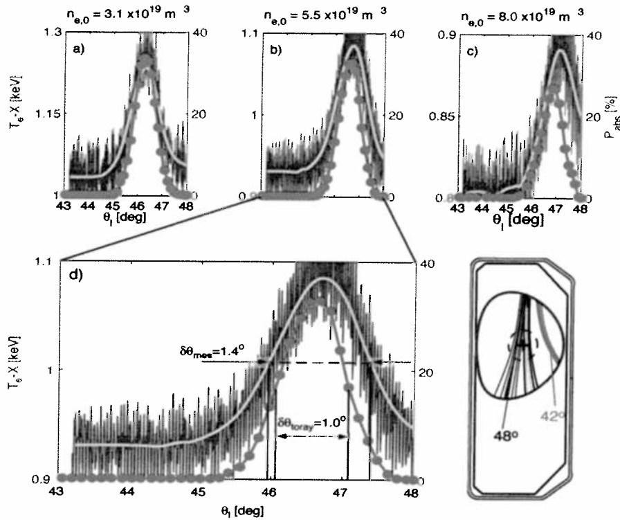
Figure 16. The global temperature deduced from the T_e -X measurement gives qualitatively the absorption efficiency (blue lines). By sweeping \theta_l , the optimal angle \theta_{l,opt} can be determined using the smoothed T_e -X signal (yellow lines). The absorption calculated by TORAY-GA is superimposed on T_e -X (red lines with dots). The poloidal view of the plasma cross-section shows the beam trajectories during the sweep. The angle sweep scenario has been repeated for three central densities a) n_{e,0} = 3.1 \cdot 10^{19} \text{ m}^{-3} , b) n_{e,0} = 5.5 \cdot 10^{19} \text{ m}^{-3} and c) n_{e,0} = 8.0 \cdot 10^{19} \text{ m}^{-3} . d) The launcher poloidal angular tolerance \delta\theta from T_e -X and P_{abs} .
