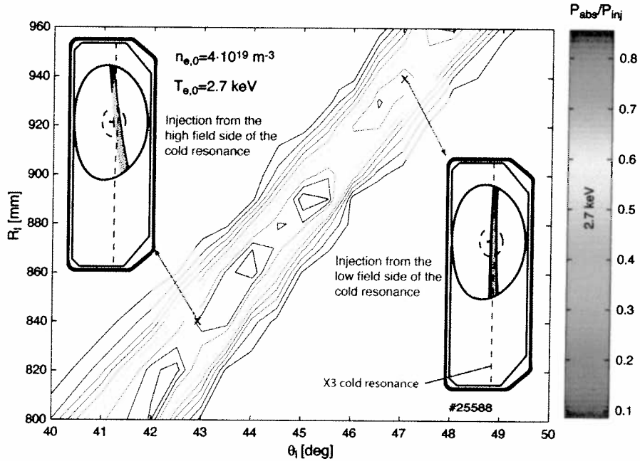
Figure 11. The contour plot of the absorption calculated by TORAY-GA in the X3 launcher parameter space, R (radial position) and \theta_l (poloidal angle), shows that an optimal angle \theta_{l,opt} can be found for any R within the accessible range. The poloidal views of TCV in the figure corners show the calculated beam trajectories for two different values of \theta_{l,opt} .
