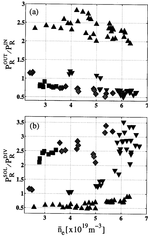
Fig. 3. Variation of the ratio P_R^{OUT}/P_R^{IN} (a) and P_R^{SOL}/P_R^{DIV} (b) with \bar{n}_e for different effective neon concentrations at I_p = 280 kA. The approximate real concentrations (in % of the total number of electrons) derived from IR Bremsstrahlung and soft X-rays are: ▲ No neon, ▼ 0.25 < C_{Ne} \leq 1.2 , ◆ 1.2 < C_{Ne} \leq 2 , ■ 2 < C_{Ne} \leq 2.5
