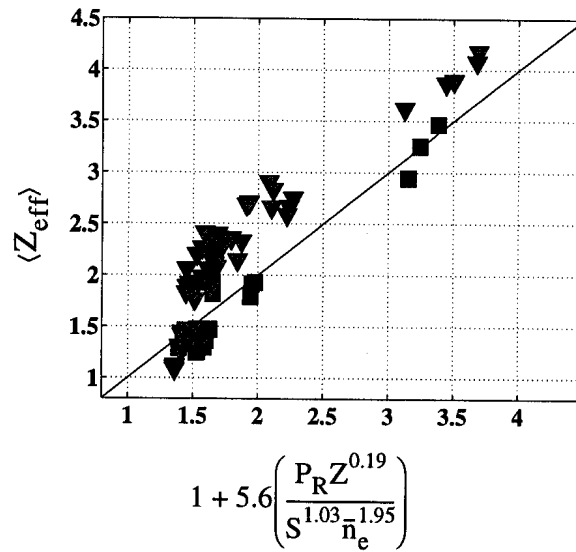
Fig. 4. Comparison of the measured volume averaged Z_{\text{eff}} with the scaling due to Matthews [1] for shots with neon injection ( Z = 10 assumed). The data are separated according to the main/edge plasma radiation distribution and include discharges at I_p = 280 kA and 380 kA.
