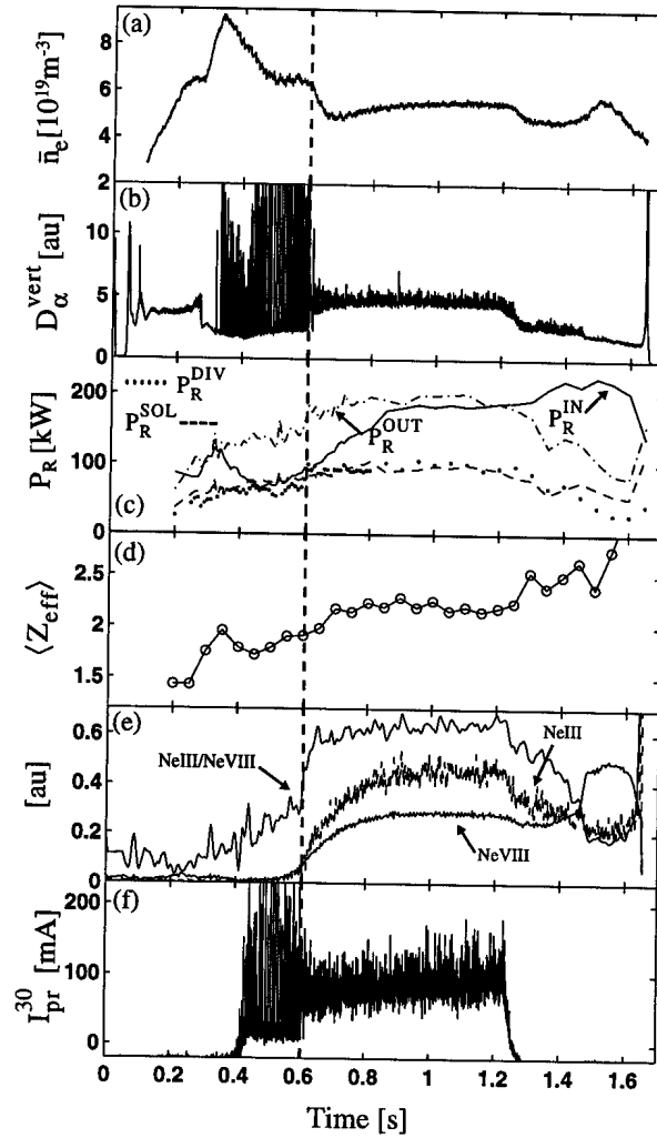
Fig. 5 TCV discharge #13459 with I_p = 380 kA in which an ohmic H-mode phase (L-H transition at t = 0.273 s) is terminated by neon injection beginning at t = 0.55 s. The time of the H-L transition is indicated by the vertical dashed line. (a) \bar{n}_e along the central chord, (b) D_\alpha for a chord passing vertically through the machine centre, (c) separated components of radiation distribution, (d) volume averaged Z_{\text{eff}} , (e) NeIII, NeVIII line intensities and their ratio, (f) I_{\text{sat}} to a target probe located 2-3 cm from the outboard strike point.
