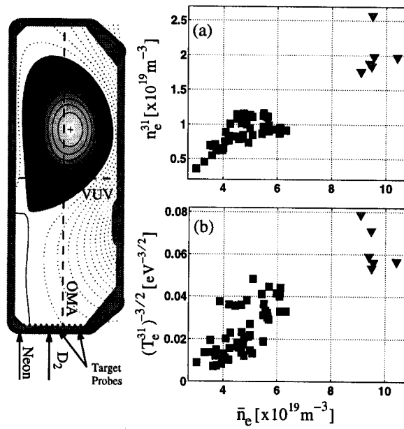
Fig. 1. Left, the SNL configuration used for the neon injection. Right, the dependence on \bar{n}_e in the absence of neon of a) n_e and b) T_e^{-3/2} for target Langmuir probe 31 located 5-6 cm from the outer strike-point. ■ I_p = 280 kA, ▼ I_p = 380 kA.
