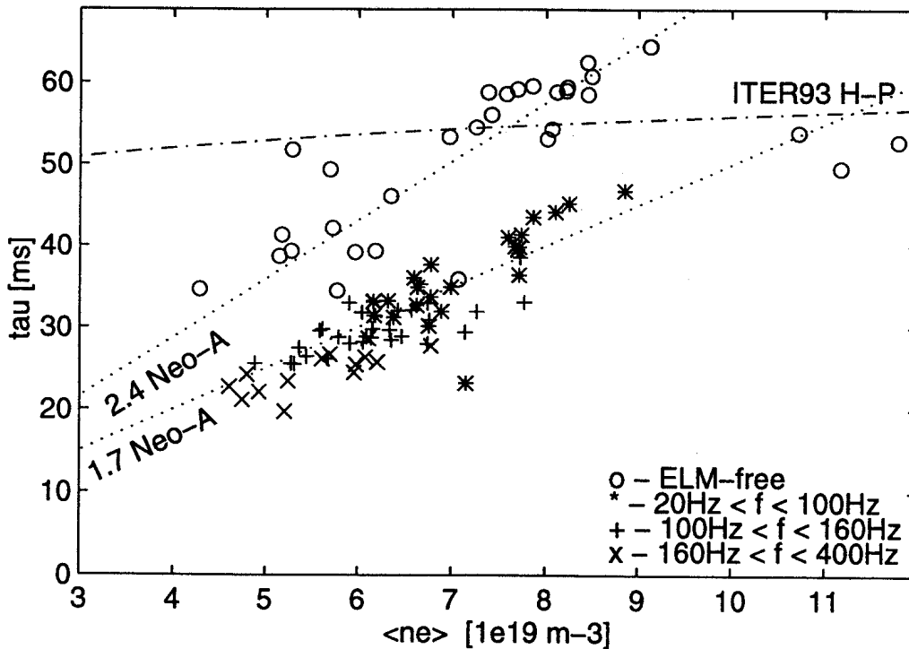
Figure 3. Energy confinement times versus line average density for Elm-free H-modes and for stationary ELMy H-modes in Single Null with I_p = 330 kA.
