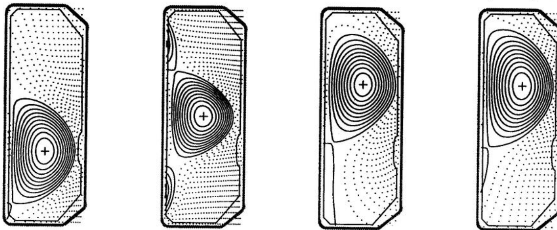
Figure 1. Selection of H-mode configurations produced in TCV
