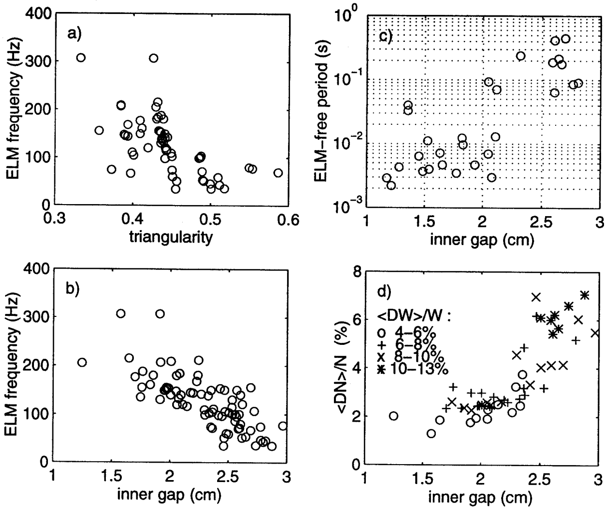
Figure 13. Effect of gap between inner wall and LCFS on ELM frequency and amplitude. a) ELM frequency versus \delta . b) ELM frequency versus gap c) Initial ELM-free period versus gap d) ELM amplitude versus gap
