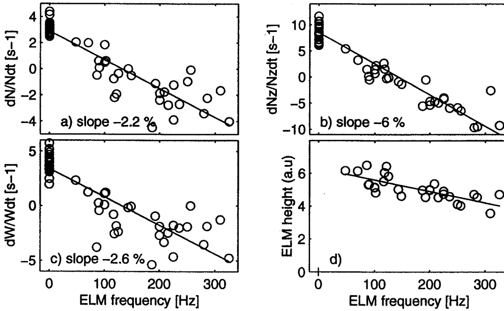
Figure 1. Rates of change of a) electron content, b) impurity content and c) stored energy versus ELM frequency in DND H-modes. d) pulse height of the D_{\alpha} emission.
