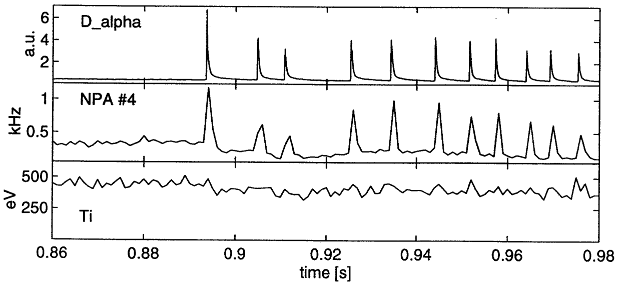
Figure 10. Charge exchange signals in ELMy H-mode. a) D_\alpha monitor b) CX count rate for 1.6 keV channel of NPA c) Ion temperature from NPA measurement (TCV shot # 8001).
