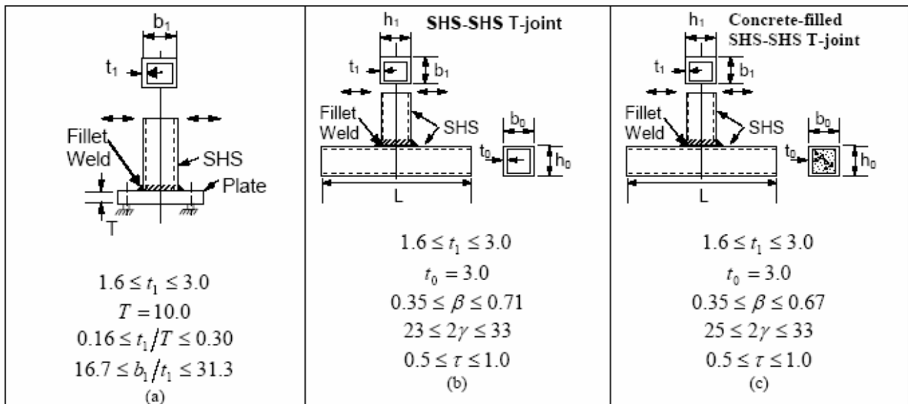
Fig. 8. (a) SHS-Plate (bolted to rigid plate), (b) Empty SHS-SHS (simply supported at both ends) and (c) Concrete-filled chord SHS-SHS T-joints under in-plane bending (simply supported at both ends)
