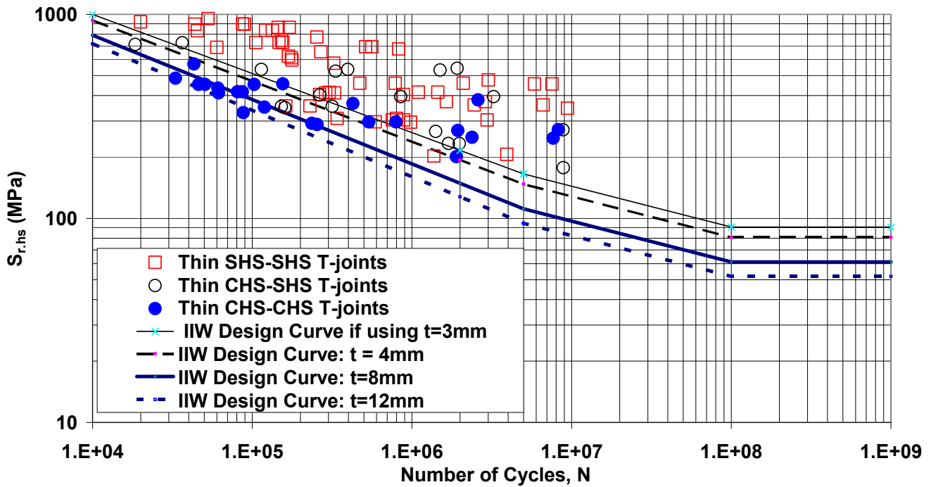
Fig. 7. Existing Design S_{r,hs} - N curves from IIW 16 and fatigue test data for welded thin-walled ( t < 4\text{mm} ) CHS-CHS, CHS-SHS and SHS-SHS T-joints.
