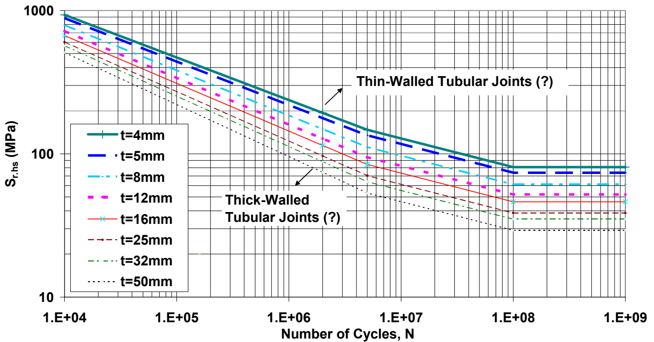
Fig. 2. Fatigue design curves for tubular nodal joints in standards 16,17 and knowledge gaps identified
