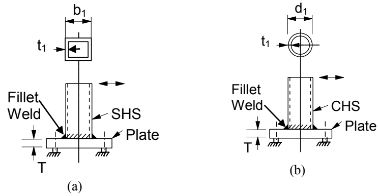
Fig. 3. (a) SHS-Plate and (b) CHS-Plate T-joints under cyclic in-plane bending (bolted to rigid plates)
