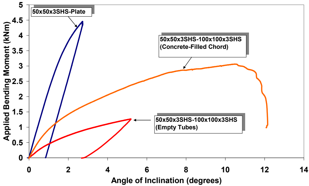
Fig. 9. Applied bending moment vs angle of inclination in joints of different stiffness
