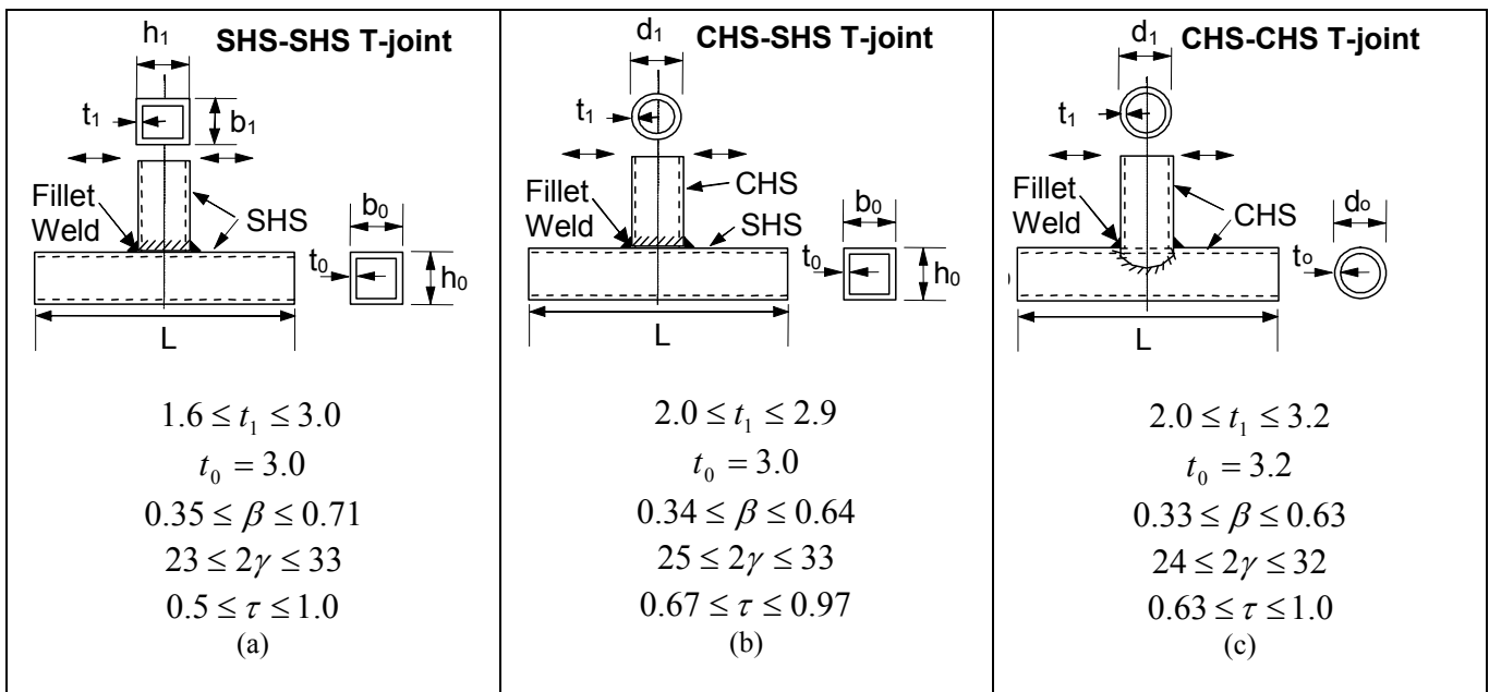
Fig. 6. (a) SHS-SHS, (b) CHS-SHS and (c) CHS-CHS T-joints under in-plane bending (simply supported at both ends)
