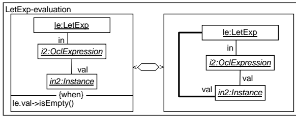
Fig. 22 Let Expression: Binding and Evaluation
