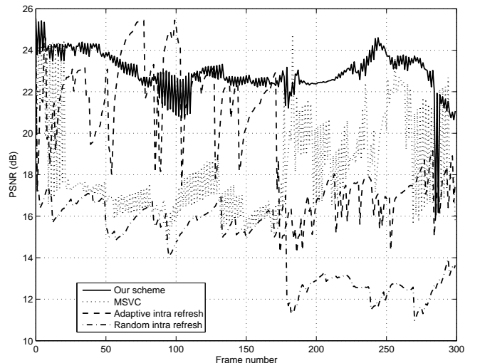
Figure 9: Reconstructed video quality, on a frame basis, when PLR = 10% (Stefan CIF, 30 fps, 512 kbits/s).
