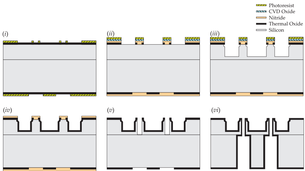
Figure 20. Microfabrication steps of capillary emitter tips.
