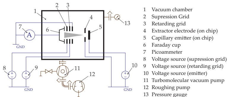
Figure 11. Schematic of the electro spray test rig.
