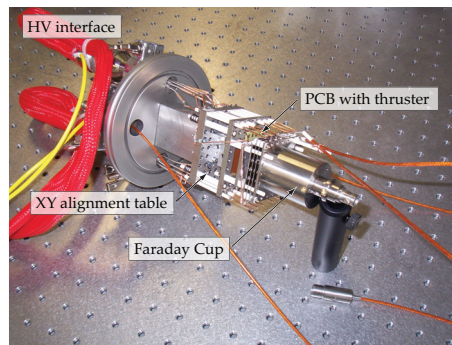
Figure 12. Thruster assembly support structure with mounted Faraday cup.
