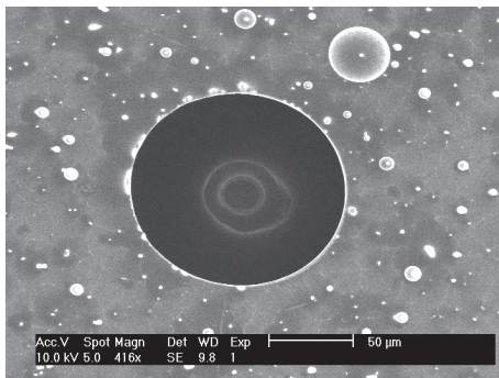
Figure 18. SEM image of droplets observed on top of the extractor electrode. Their provenance could be from the reflected beam during retarding potential measurements.
