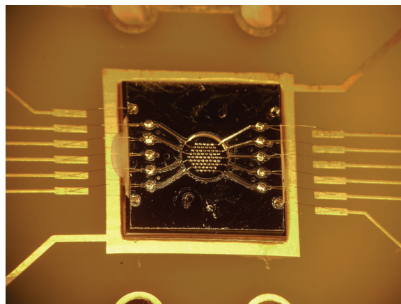
Figure 17. Thruster chip assembly with individually addressable electrodes mounted on a printed circuit board. The electrical contact between chip and PCB is done through wire bonding.
