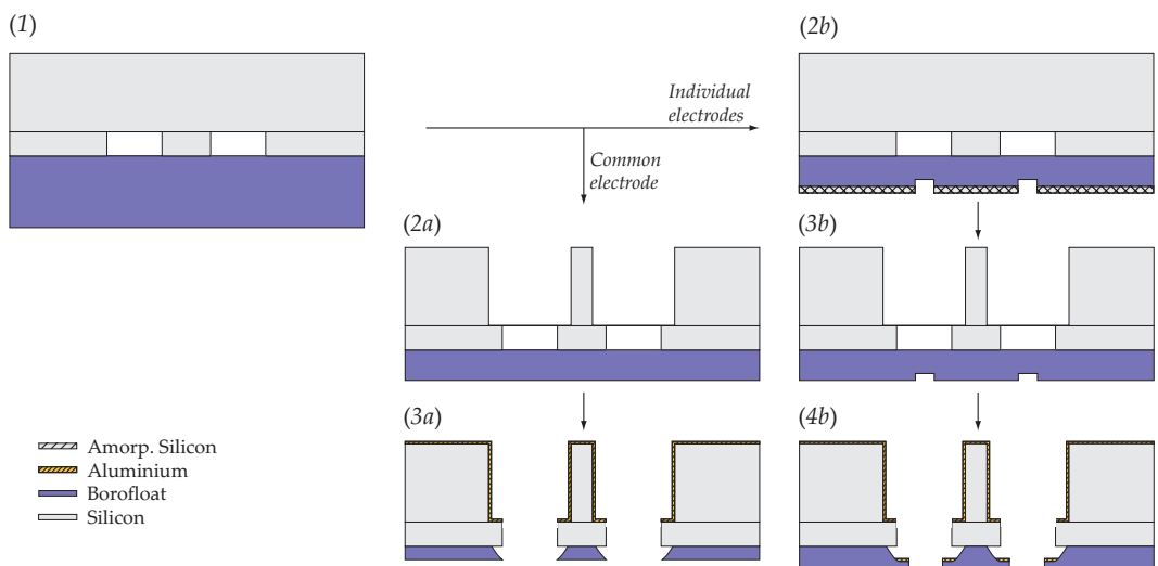
Figure 21. Microfabrication steps of extractor electrodes.
