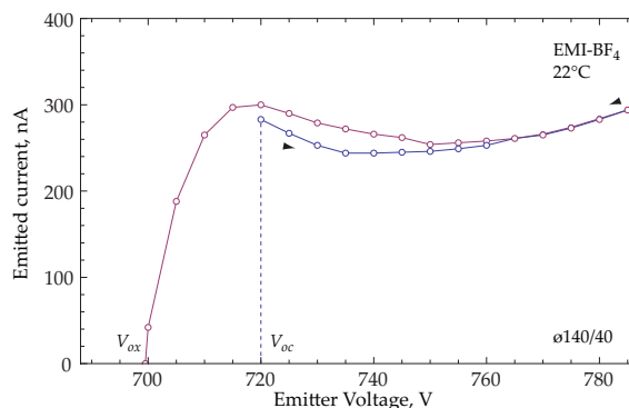
Figure 14. Current-voltage curve for EMI-BF 4 of a capillary with 20\mu\text{m} i.d. and a 140\mu\text{m} diameter electrode spaced. 40\mu\text{m} from the emitter
