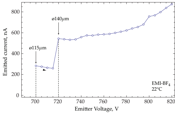
Figure 15. Current-voltage curve for EMI-BF 4 of two capillaries with 20 μm i.d. with the extraction electrode spaced 40 μm from the emitters. The jump in current is due to the different starting voltages of an extractor with 115 and one with 140 μm diameter
