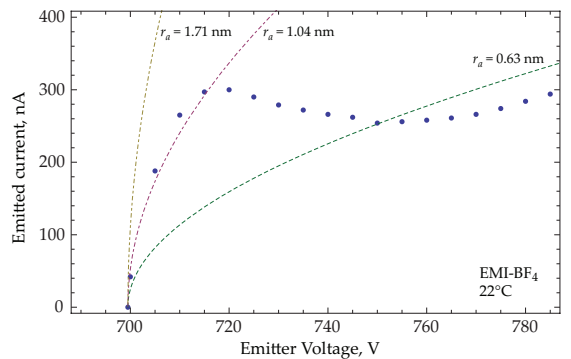
Figure 19. Overlay between a measured current-voltage curve and several calculated ones. The analytical model assumes a purely ionic regime whereas the measured beam contains most likely droplets.
