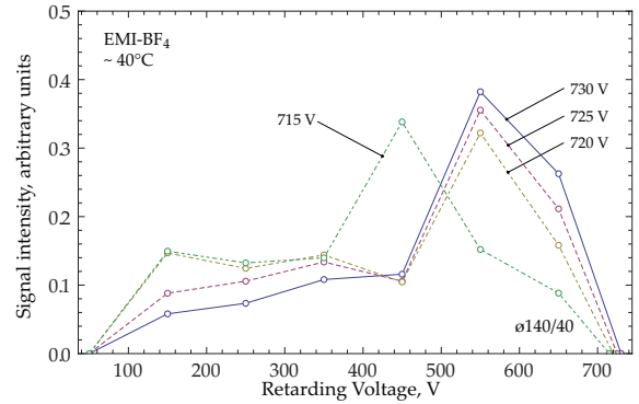
Figure 16. Retarding potential measurement of a capillary with 140 μm extractor electrode at 40 μm from the emitter. Measurements were taken for different operation voltages
