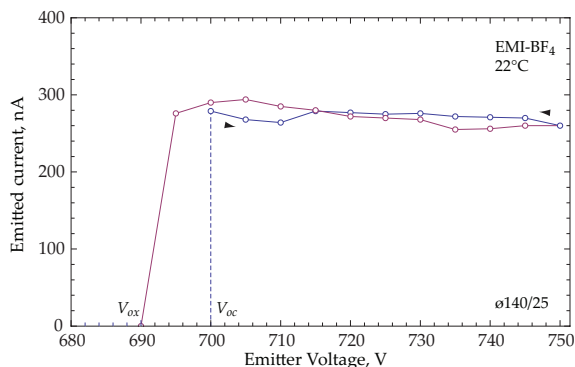
Figure 13. Current-voltage curve for EMI-BF 4 of a capillary with 20\mu\text{m} i.d. and a 140\mu\text{m} diameter electrode spaced. 25\mu\text{m} from the emitter
