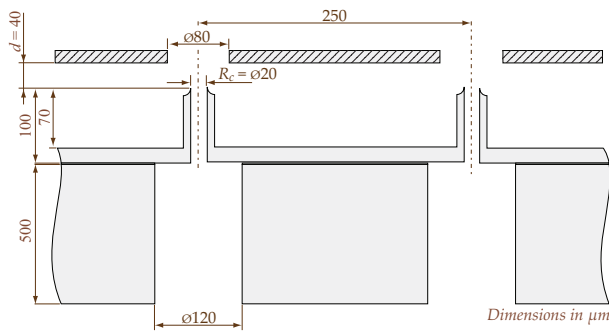
Figure 3. Geometry of the capillaries.
