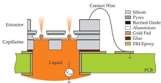
Figure 1. Schematic cross-section of the experimental assembly.
