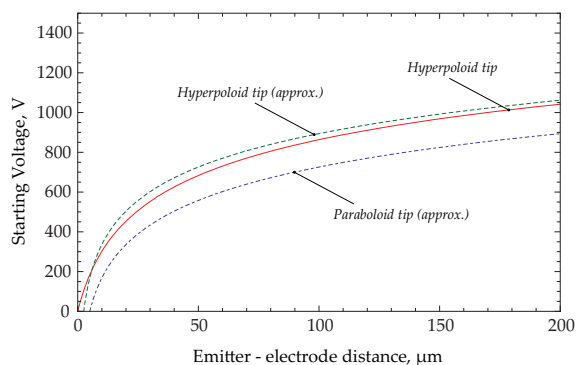
Figure 2. Estimated starting voltage for a hyperboloid tip model and a paraboloid tip model.
