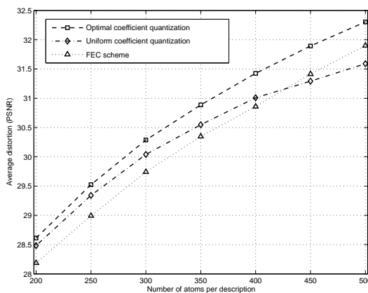
Fig. 3. Minimal achievable average distortions, as a function of number of atoms per description.
