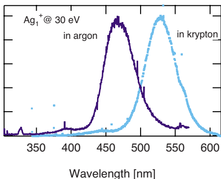
FIG. 9. (Color online) Spectrally resolved luminescence of Ag_1^+ , during the deposition in an argon and a krypton matrix.
