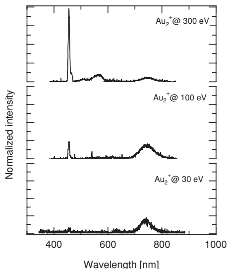
FIG. 10. Spectrally resolved luminescence of Au_2^+ , during the deposition into an argon matrix. The comparison with Fig. 8 shows that when the impact energy is raised the gold dimer fragments. The fact that we observe the luminescence of the fragment means that the luminescence process happens after the fragmentation has taken place. The spectra are normalized in order to keep the area below them constant.
