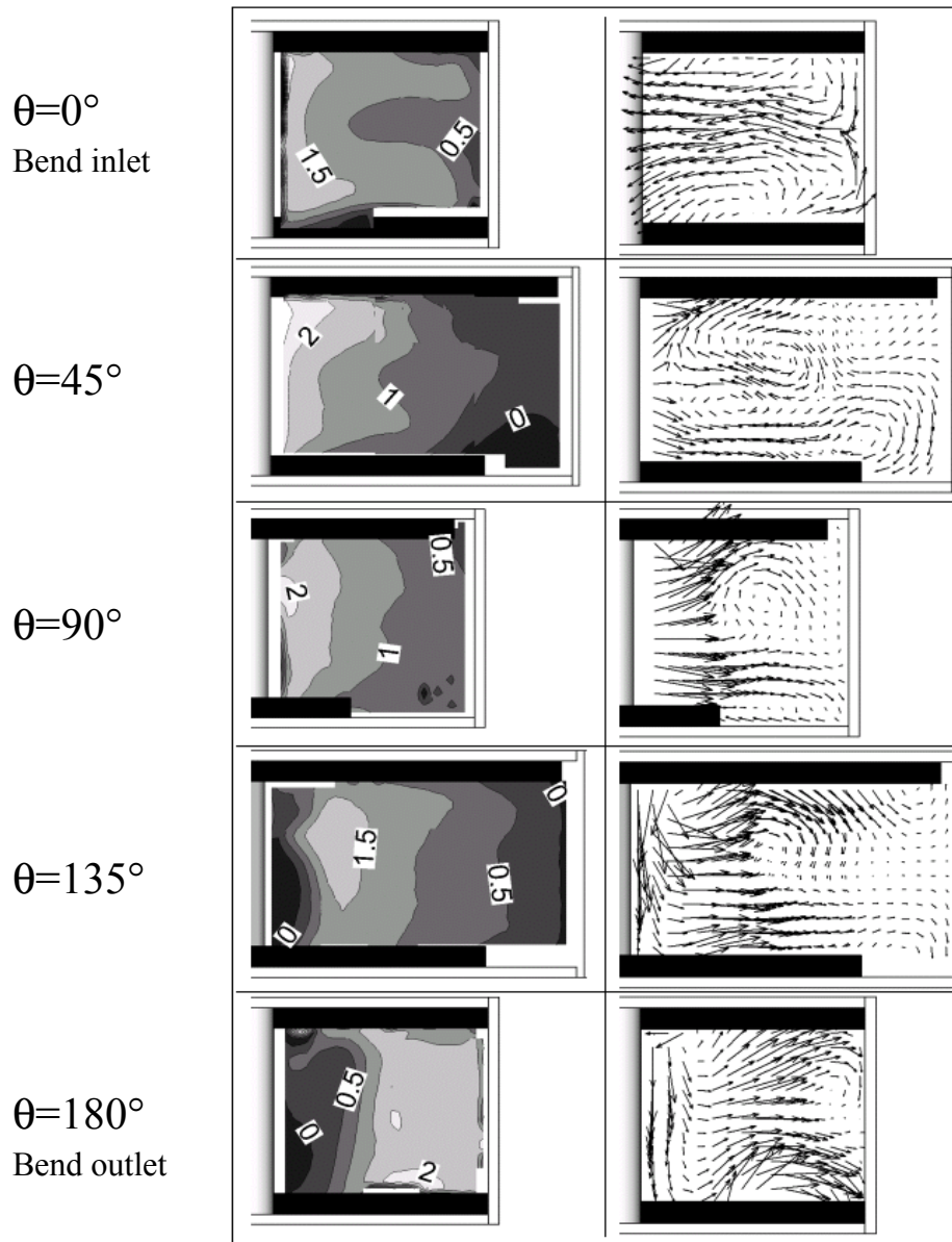
Figure 5: Mean streamwise velocity contours and secondary flow vectors obtained at \theta = 0, 45, 90, 135 and 180 deg in the bend. The contour lines values, U_\theta , are plotted on the figures ( U_\theta / U_b ).
