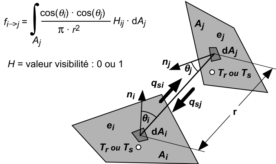
2-37 Condition aux limites de type "radiosité"
