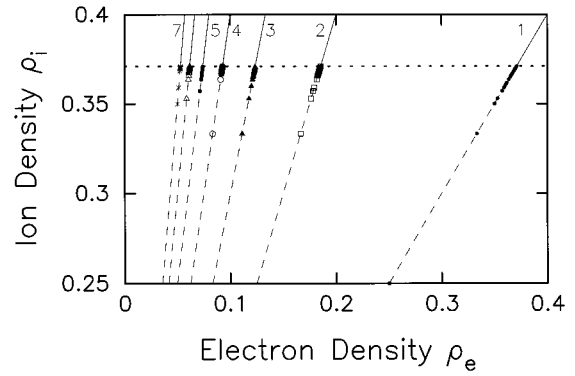
FIG. 1. Stable periodic configuration for n molecules, i.e., states with \rho_i = n\rho_e . The values n=1 (solid dot), n=2 (open square), n=3 (solid triangle), n=4 (open dot), n=5 (solid square), n=6 (open triangle), and n=7 (x) are all plotted. The phases are stable above \rho_c as indicated by the solid lines. The dashed lines are guides to the eye.
