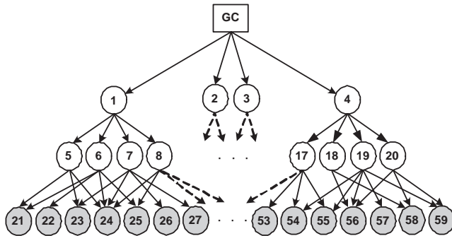
Figure 4: Tree structure for multiview pose detection. GC is built using HF. All the other pose specific classifiers use GF.
