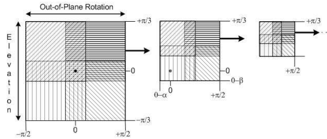
Figure 3: Hierarchical sampling of the pose plane.
