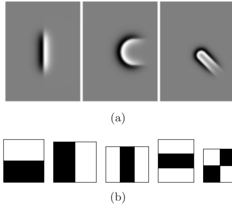
Figure 2: Filters used for modeling the faces: 2(a)Anisotropic Gaussian and 2(b)Haar-like filter.
