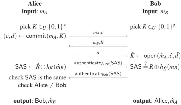
Fig. 4. A New SAS-Based Message Cross-Authentication Protocol.
