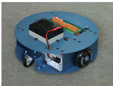
Figure 3: Robotic platform.
