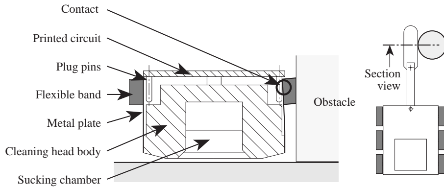
Figure 6: Section view of the tactile sensor.
