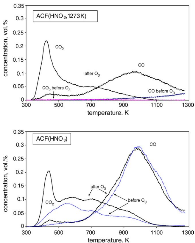
Fig. 5. TPD profiles obtained with the ACF samples (0.06 g) before and after ozone decomposition for 12 h.
