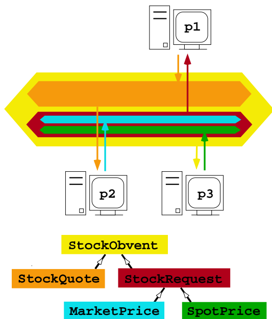
Figure 1. Type-based publish/subscribe
