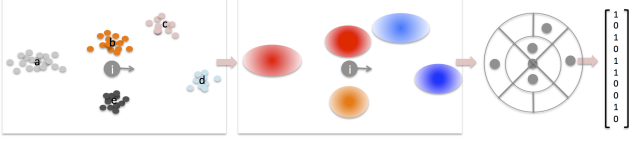
Figure 4: Illustration of a Social Affinity Map extraction (top view). The relative positions of neighboring individuals are clustered into a radial histogram. The latter is one bit quantized.
