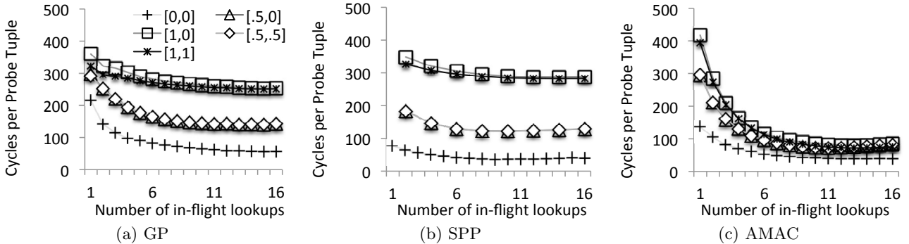
Figure 6: Probe performance sensitivity to GP, SPP, AMAC tuning parameters on Xeon x5670 ( 2GB \bowtie 2GB ).
