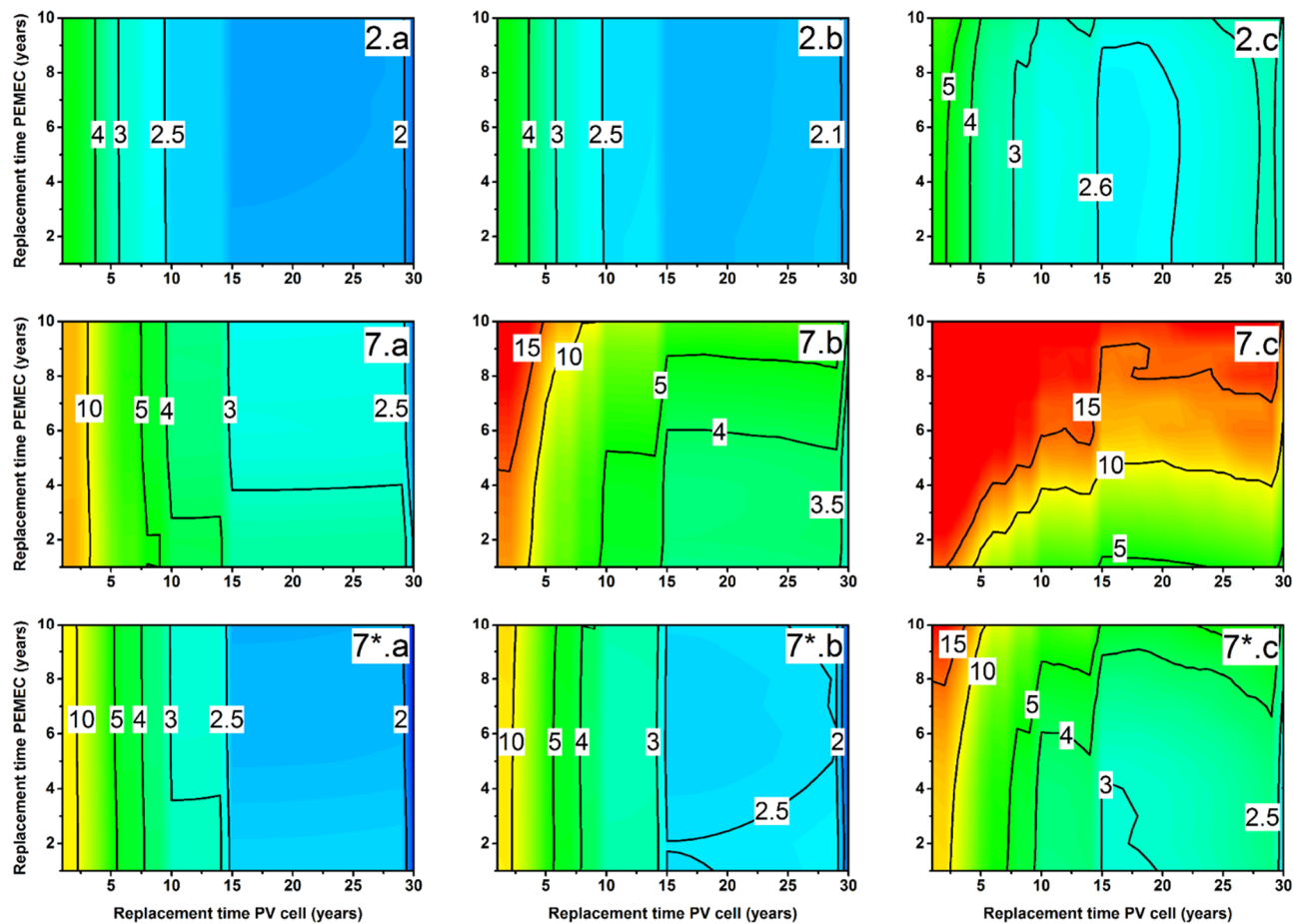
Figure S5. Hydrogen price p_{\min} (in \$/\text{kg}_{\text{H}_2} ) as a function of replacement time of PV cells and PEMEC for cost-optimized devices 2, 7*, and 7, for (a) optimistic, (b) reference, and (c) conservative degradation rates.
