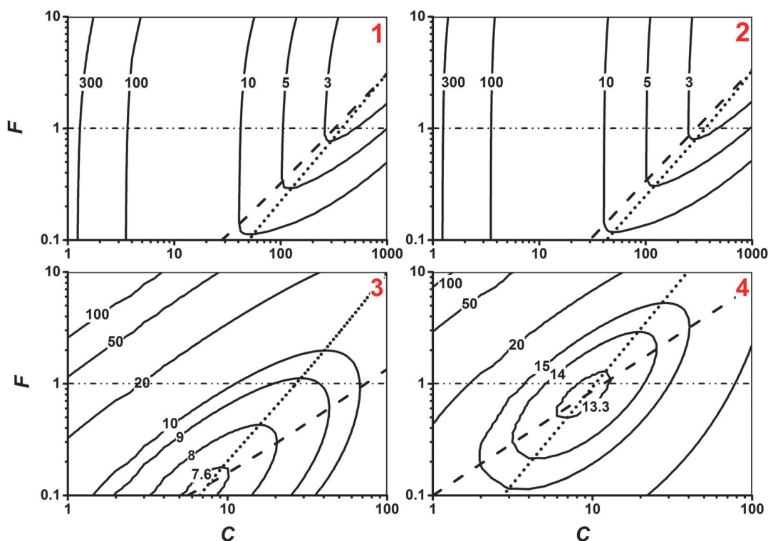
Fig. 3 p_{min} (in \$ \text{ kg}_{\text{H}_2}^{-1} ) as a function of F and C for concentrating device types 1–4. The dot-dashed line at F = 1 indicates the design space of device subtypes 9–12. Optimum F for a given C is shown by the dashed line, optimum C for a given F is shown by the dotted line. Minimum hydrogen prices ( \$2.03 \text{ kg}_{\text{H}_2}^{-1} , \$2 \text{ kg}_{\text{H}_2}^{-1} , \$7.54 \text{ kg}_{\text{H}_2}^{-1} , \$13.2 \text{ kg}_{\text{H}_2}^{-1} for devices 1, 2, 3, and 4, respectively) are reached at the cross point between these two curves ( C = C_{opt} = 1000 and F = F_{opt} = 3.2 for devices 1 and 2, C = C_{opt} = 7 and F = F_{opt} = 0.12 for device 3, and C = C_{opt} = 9 and F = F_{opt} = 0.74 for device 4). Minimum hydrogen prices for designs 9–12 ( C = C_{opt} = 400, 380, 28 and 11) are given by the intersection of the dotted and the dot-dashed lines at F = 1 .
