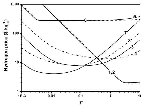
Figure S2. Hydrogen price as a function of current concentration, F , for devices 1 to 4 at C_{\text{opt}} , and for devices 5 to 8, at C=1 using high quality (solid lines) or low cost electrocatalysts (dashed lines).
