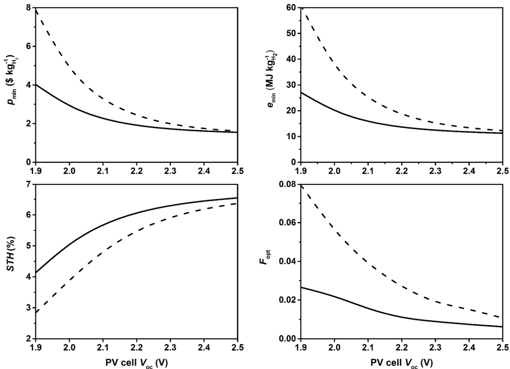
Figure S3. Evolution of p_{\text{min}} , e_{\text{min}} , \text{STH}_{\text{max}} , and F_{\text{opt}} with the PV cell's V_{\text{oc}} of device 7 (solid line) and 8 (dashed line). Device types 7 and 8 with V_{\text{oc}} = 2.5 represent device types 7* and 8*.
