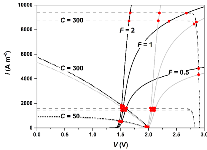
Figure S1. Typical current-voltage behavior of the device for varying C and F . The current is normalized by the area of the PV cell. The current density-voltage characteristic of the Ga-based cells (dashed lines) and the Si-based cells (dotted lines) are shown for C = 50 and 300 . Pt is used as electrocatalysts in the PEMEC, for which current-voltage behavior for F = 0.5, 1, and 2 (solid lines) at initial operating time (black lines) or after 10 years operation (gray lines) is shown. At large C and small F , mass transport limitations in the PEMEC decrease the operating current. Operating voltages and currents are given at the intersection of the PEMEC and PV cell curves and are indicated by red dots.
