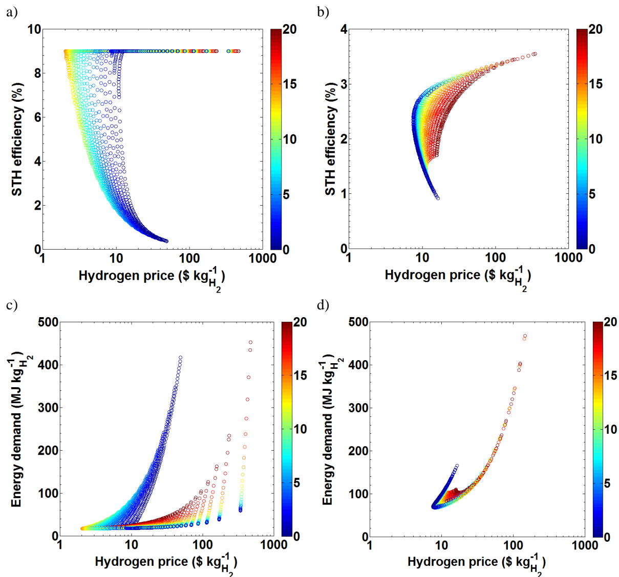
Figure S4. Operating time-averaged efficiency as a function of hydrogen price (a,b) and energy demand as a function of hydrogen price (c,d) for device types (a,c) 1 and (b,d) 3. The color of the points indicates a normalized current concentration ( [\log_{10}(F)+1] \cdot 10 ).
