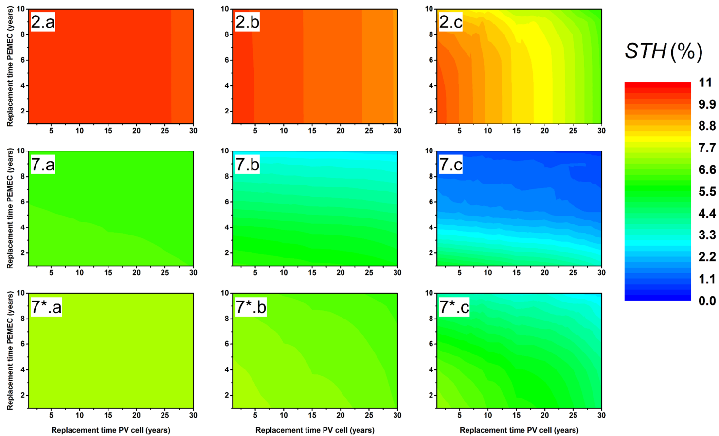
Figure S6. Operating time-averaged STH efficiency as a function of the replacement time of PV cells and PEMEC for cost-optimized devices 2, 7*, and 7, for (a) optimistic, (b) reference, and (c) conservative degradation rates.
