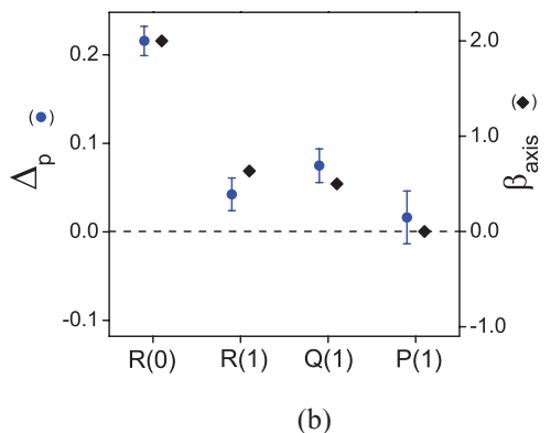
FIG. 7. Comparison of the experimentally determined \Delta_p values for \text{CH}_4(\nu_3) to (a) the corresponding calculated \bar{J} alignment coefficients A_0^{(2)} . (b) the corresponding calculated vibrational alignment coefficients \beta_{axis} . Error bars represent \pm 2\sigma of the average of 4–9 replicate measurements.
