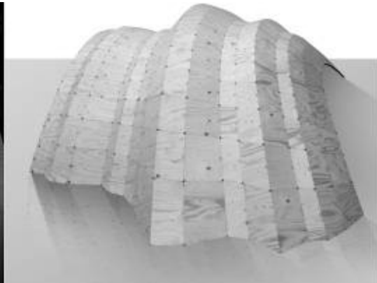
Figure 3 . Generated spatial structure made out of block timber panels
