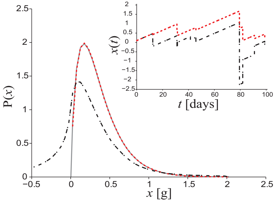
FIG. 2: Comparison of the steady state PDF of Eq.(17): S solution (solid line, obtained analytically from Eq.(18)), I solution (dash-dot, from numerical simulation), I solution using the jump distribution given by Eq.(20) (dotted line, from numerical simulation). The numerical simulations confirm our analytical results. Inset: simulated trajectory of the salt mass under the two different prescriptions. Note that if artificial reflecting barriers are not imposed, the salt mass given by the I prescription of Eq.(17) may assume unphysical negative values. The parameters used for the simulation are \mu = 0.463 , \nu = 0.15 \text{ day}^{-1} and \Upsilon = 30 \text{ mg/day} .
