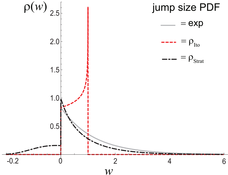
FIG. 3: Comparison between a jump exponential distribution \rho(w) with mean 1/\gamma = 0.8 , and the solutions \rho_I(z) , \rho_S(z) of the prescription induced jumps corresponding to Eqs.(20) and (21) respectively, corresponding to the given \rho(w) .
