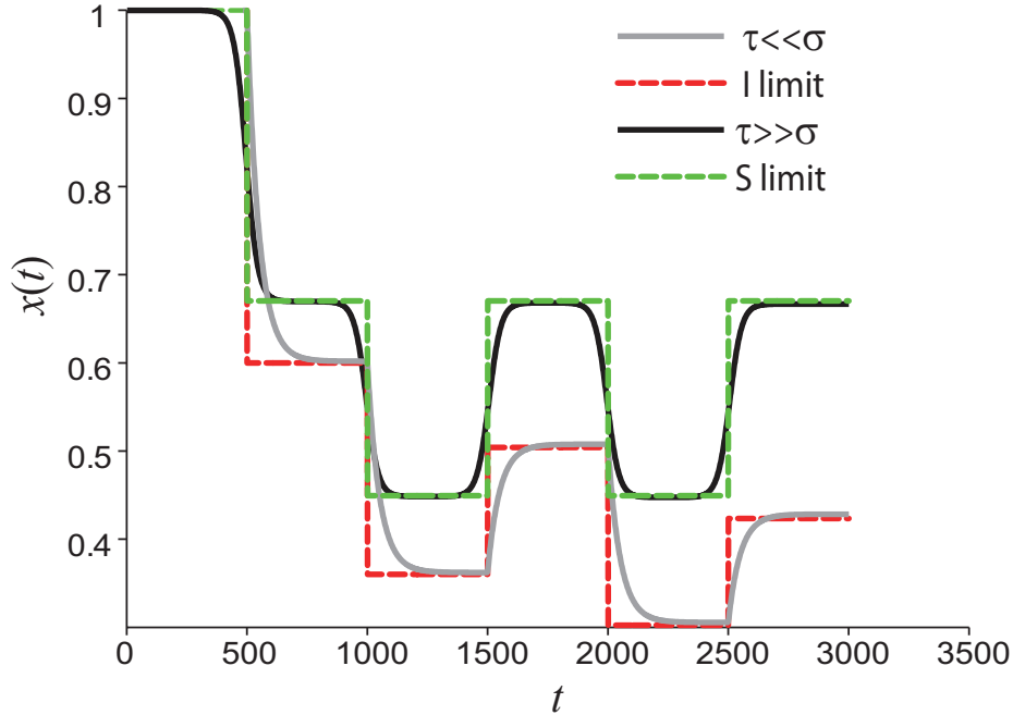
FIG. 1: Comparison between trajectories of a particle that undergoes impulsive multiplicative forcing in a viscosity field for different timescales ( \tau and \sigma ), and the trajectories that result from the SDE \dot{x}(t) = -x(t) \sum_{i=1}^5 w_i \delta(t - t_i) interpreted in the I and S prescriptions. The jumps in this case are given by w_i = \pm 0.4 .
