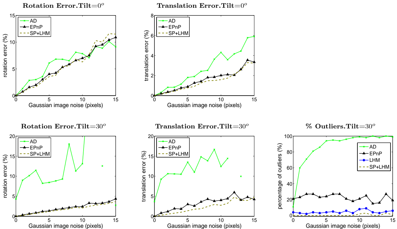
Fig. 7 Planar case. Errors as a function of the image noise when using n = 6 reference points. For \text{Tilt}=0^\circ , there are no pose ambiguities and the results represent the mean over all the experiments. For \text{Tilt}=30^\circ , the errors are only averaged among the solutions not affected by the pose ambiguity. The right-most figure represents the number of solutions considered as outliers, which are defined as those for which the average error in the estimated 3D position of the reference points is larger than a threshold.
