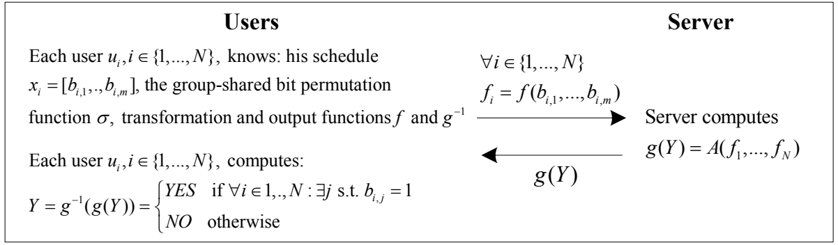
Figure 1: A generic scheduling protocol. Users first send their transformed schedules f_i to the server, which then performs the scheduling algorithm A on the received data and sends the encrypted output g(Y) back to each user.
