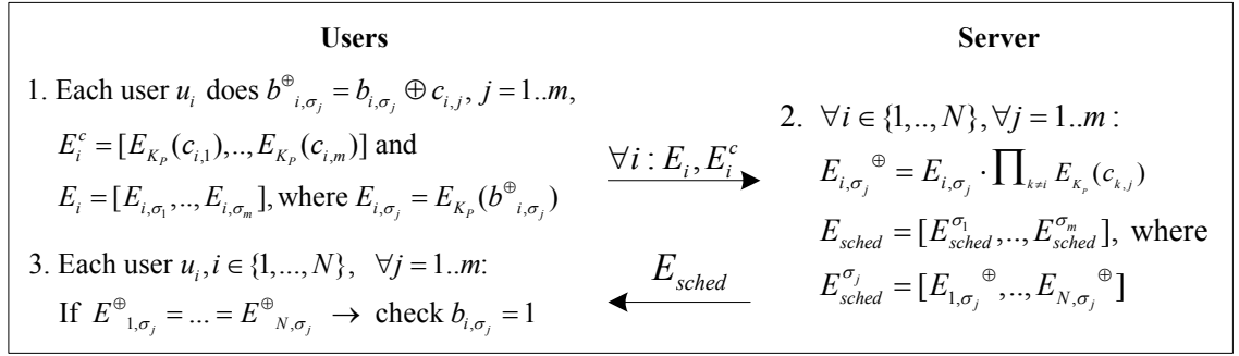
Figure 5: SchedGM protocol.
