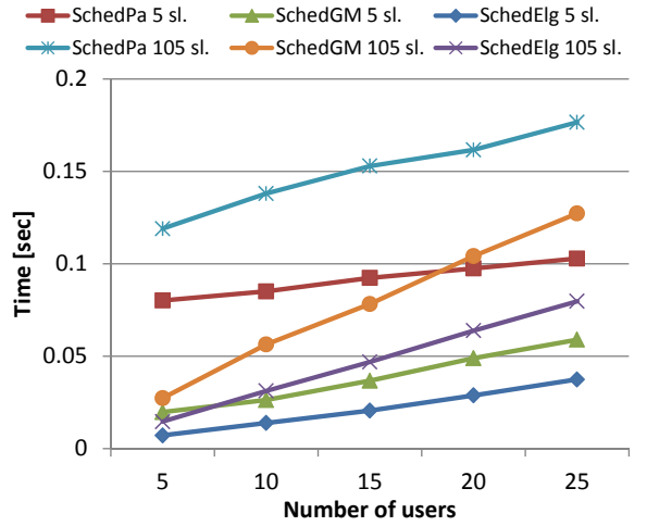
Figure 8: Server processing performance.
