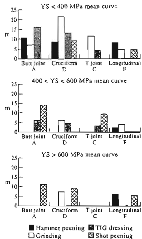
Fig. 2. Values of m deduced from mean curves (linear regression \log \Delta\sigma - \log N )
