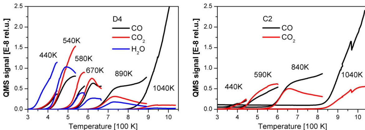
Fig. 5 – Step-wise TPD profiles of CO (black line) and CO_2 (red line) evolution from the samples D4 (ozone activated, left) and C2 (hydrogen peroxide activated, right). For sample D4 also the traces of water without background subtraction are shown.
