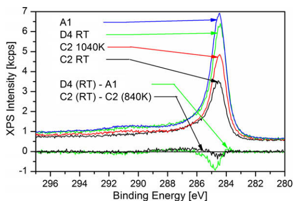
Fig. 2 – C1s spectra normalized at the minimum of the intensity between the C1s and its Mg satellites of the untreated CNF/SNF Inconel sample A1, the functionalized samples C2 ( \text{H}_2\text{O}_2 ) and D4 ( \text{O}_3 ) before heating and additionally C2 after heating to 1040 K in UHV. In the lower part difference spectra of oxidized/untreated sample (D4 (RT) – A1), and oxidized/heated sample (C2 RT – C2 840 K) are shown.
