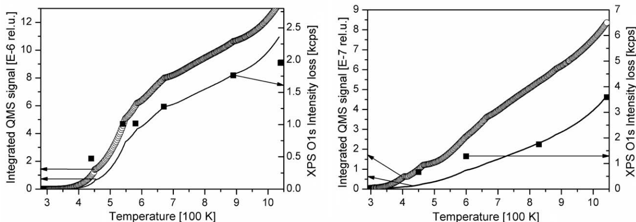
Fig. 7 – Two integrated TPD profiles for oxygen in CO and CO 2 (line) and H 2 O, CO and CO 2 together with XPS O1s loss of samples D4 (ozone activated, left) and of sample C2 (hydrogen peroxide activated, right). The XPS and TPD intensities are adjusted in the high temperature range (800–900 K) of the integrated TPD profile without water. Direct quantification and exact adjustment are hampered, due to the different probing depths of the two methods.
