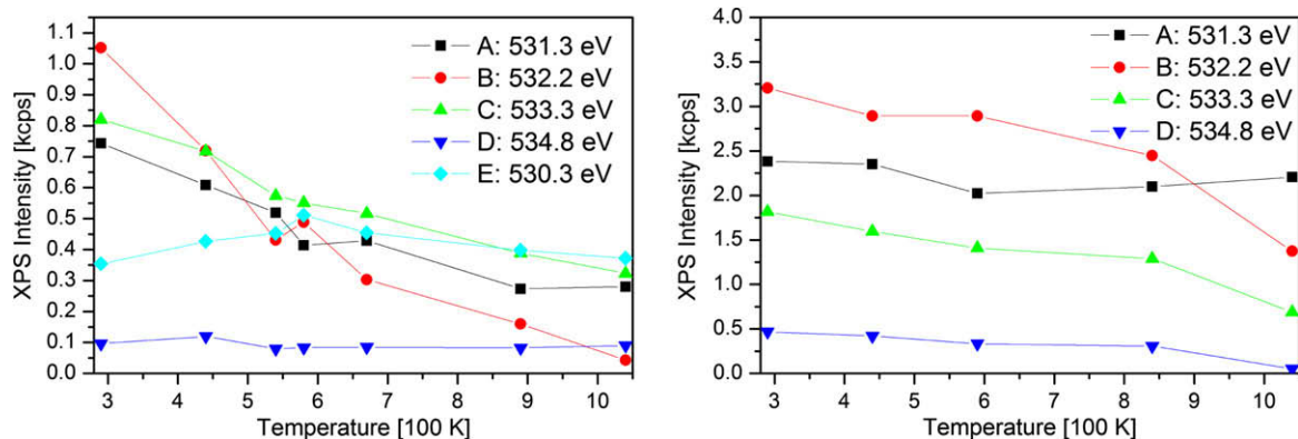
Fig. 6 – Development of the XPS O1s decomposition functions in the spectra of the samples D4 (O 3 , left) and C2 (H 2 O 2 , right) during step-wise heating under UHV.
