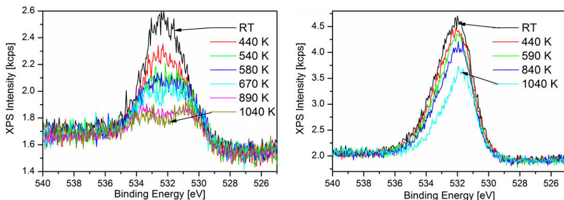
Fig. 3 – Development of the XPS O1s spectra of the samples D4 ( O_3 , left) and C2 ( H_2O_2 , right) during step-wise heating until 1040 K. The spectra are unrefined, but aligned at the minimum of the intensity between the O1s and its Mg satellites.
