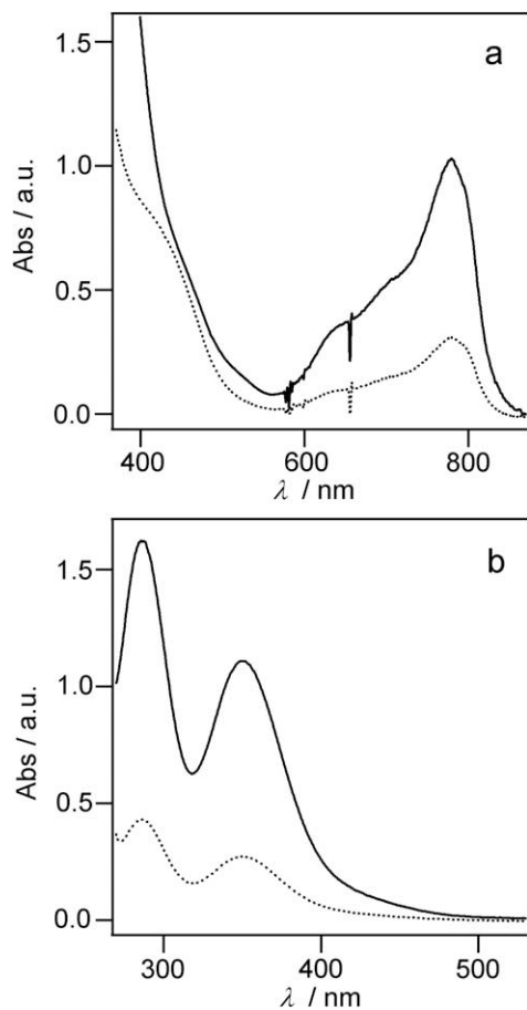
Fig. 4. UV-visible spectra of DCE solution (a) and aqueous solution treated by excess NaI (b) after biphasic stirring 20 min using TMA + as a common ion (5 mM TMAcI in water and 50 mM TMATB in DCE). The aqueous phase contained 10 mM HCl in all three cases. The DCE phase contained: 5 mM DMFc (dotted), 0.1 mM DA and 5 mM DMFc (full).
