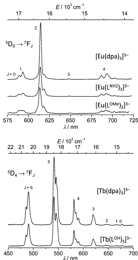
Figure 1. Three-photon excited ( \lambda_{\text{ex}} = 800 nm) luminescence spectra for Eu III and Tb III dipicolinates and their derivatives in Tris–HCl (pH 7.4, c = 10 mM). Spectral intensities are relative to [Ln(dpa) 3 ] 3- .
