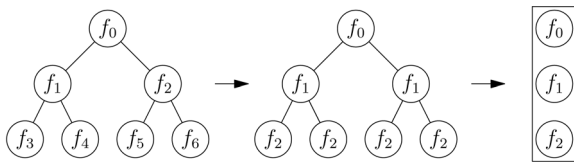
Fig. 4. Ferns versus trees. A tree can be transformed into a fern by performing the following steps. First, we constrain the tree to systematically perform the same test across any given hierarchy level, which results in the same feature being evaluated independently of the path taken to get to a particular node. Second, we do away with the hierarchical structure and simply store the feature values at each level. This means applying a sequence of tests to the patch, which is what ferns do.
