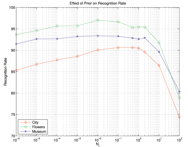
Fig. 3. Recognition rate as a function of \log(N_r) using the three test images of Section 4. The recognition rate remains relatively constant for 0.001 < N_r < 2 . For N_r < 0.001 , it begins a slow decline, which ends in a sudden drop to about 50 percent when N_r = 0 . The rate also drops when N_r is too large because too strong a prior decreases the effect of the actual training data, which are around 10,000 samples for this experiment.
