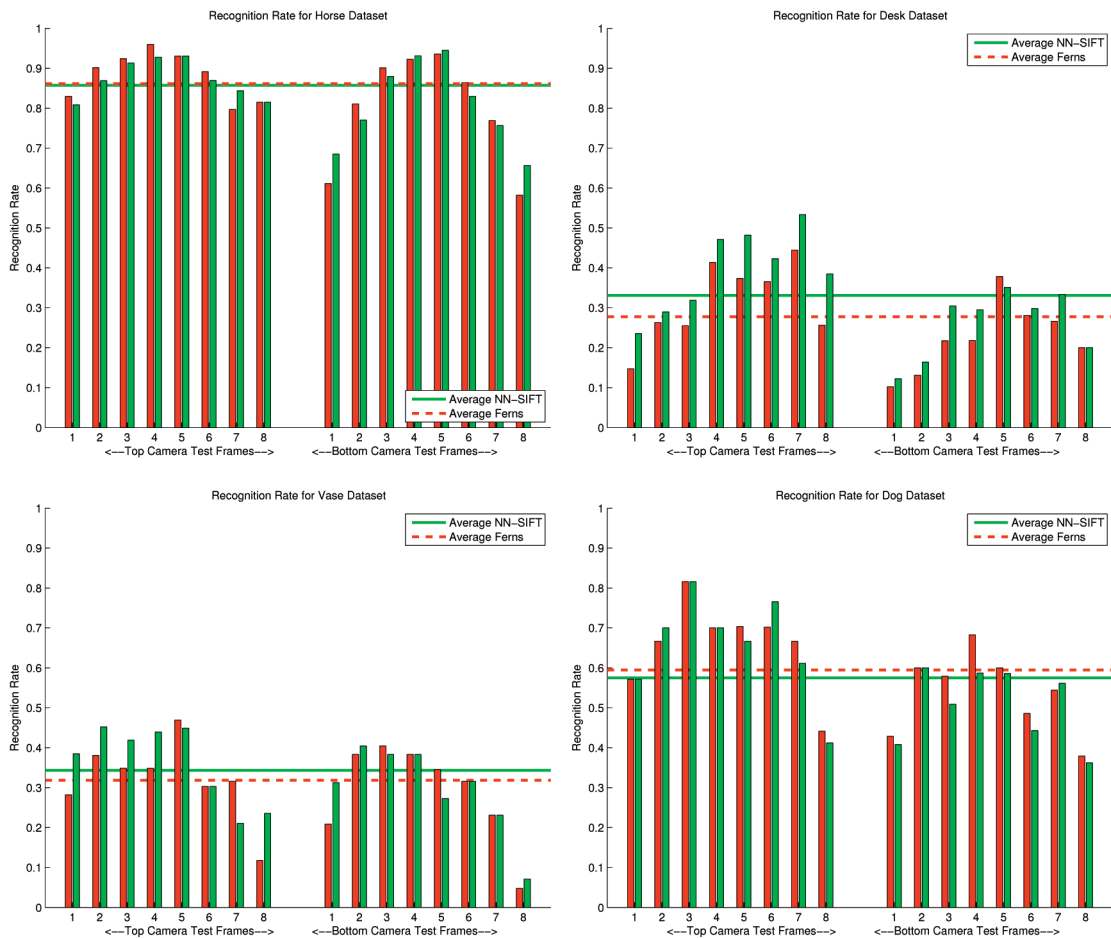
Fig. 15. Recognition rates for 3D objects. Each pair of bars corresponds to a test frame. The red bar on the left represents the rate for ferns and the light green bar on the right for Nearest-Neighbor SIFT matching. The weighted averages over all frames also appear as a dashed line for ferns and solid line for NN-SIFT. The weights we use are the number of keypoints per frame.
