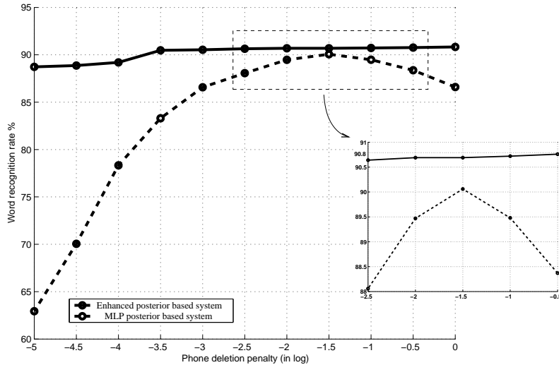
Figure 8: Comparing the sensitivity to tuning phone deletion penalty, for the decoder using enhanced posteriors and the one using MLP posteriors. Phoneme deletion penalty is varied for the two decoders and the performances are observed (on OGI Numbers’95 database). The inside diagram is a zoom of performance curves for small values of phone deletion penalty (fine tuning). The decoder using enhanced posteriors is much less sensitive to tuning ad-hoc parameters than the one using regular MLP posteriors.
