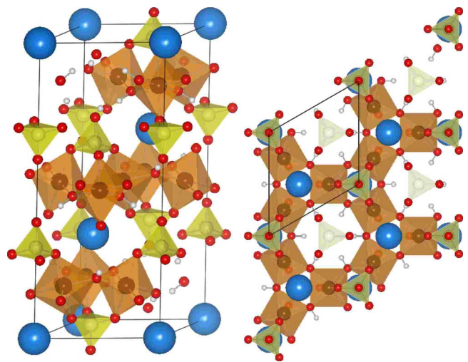
FIG. 1. (Color online) The jarosite structure viewed perpendicular to the c axis (left picture) and along the c axis (right picture), revealing the kagome network of magnetic ions. The \text{MO}_6 octahedra are drawn in transparent dark gray (brown) with the M^{3+} ions at the center (dark brown). The \text{SO}_4 tetrahedra are transparent light gray (yellow). The large spheres at the origin of the unit cells (blue) are the A site ions and the hydrogen of the \text{OH} groups are drawn as small white spheres.
