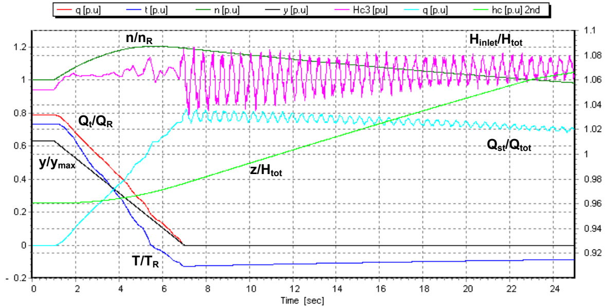
Fig. 4 Evolution of the turbine 1 variables during total load rejection
