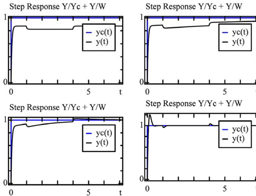
Figure 5: Increasing effect of the integrator term on set-point tracking and disturbance rejection in PI control.
