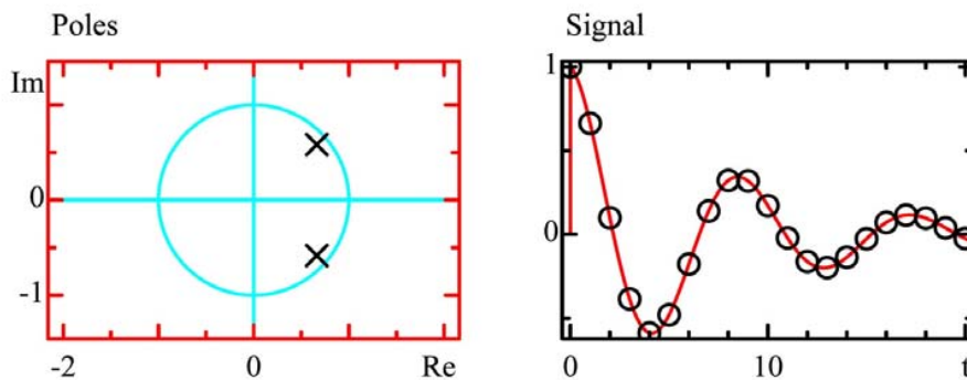
Figure 2: Relationship between poles and time response (two stable complex conjugate poles).
