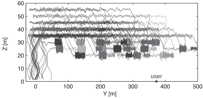
Fig. 9 Side view of the trajectories of each MAV in the swarm over the deployment, maintenance and retraction trial shown in Fig. 8. The MAVs, are launched and land around Y=0 . Node-MAVs navigate at altitudes of 20, 25, and 30 m which can be seen by the compact orbiting trajectories at these altitudes, the ant-MAVs on the other hand fly above the grid.
