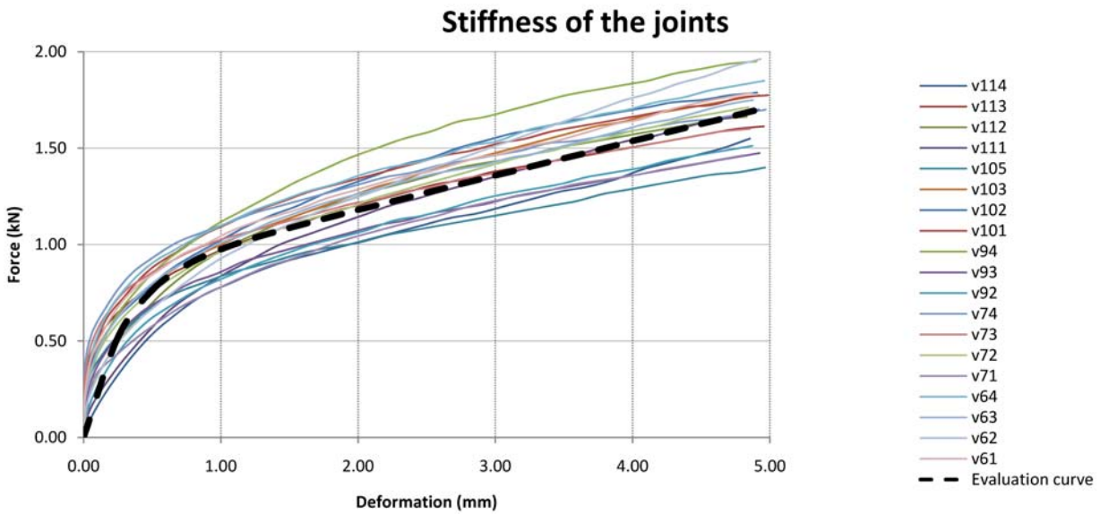
Fig.12. Shear stiffness of the joints with screws d=4.0 , l=80\text{mm} Assy Ecofast
