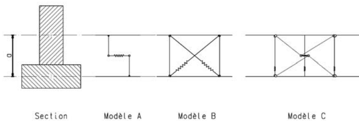
Fig.4. Framework models
