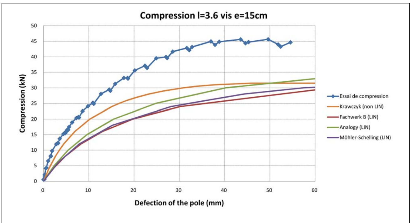
Fig.16. Compression-deflection simple normal force loaded 6-layerde pole
