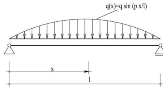
Fig.3. 2 Statical system
