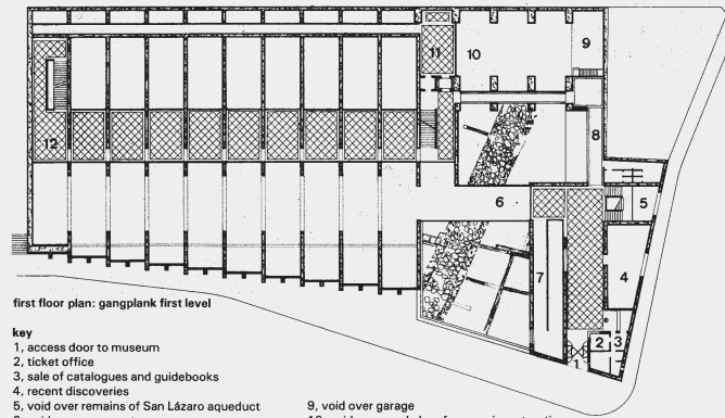
Plan niveau +1
